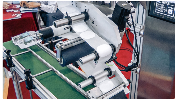
Automatic equipment for self-adhesive labels on top of pharmaceutical production
