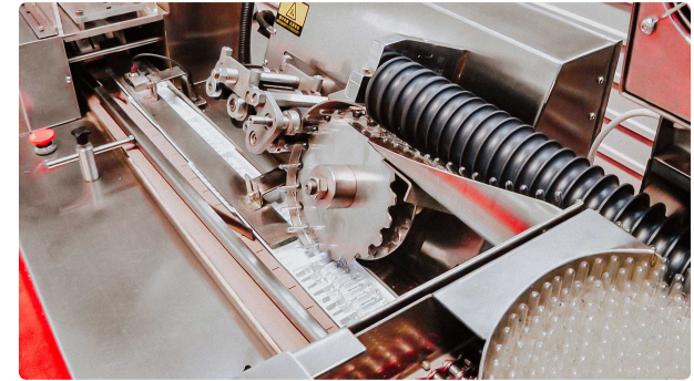
Automatic packaging machine for stacking glass ampoules in plastic blisters
