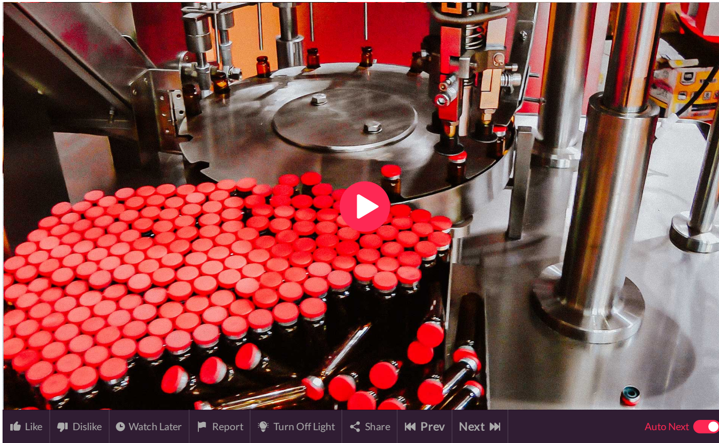
Automatic bottling and capping machine penicillin bottles with aluminum caps
