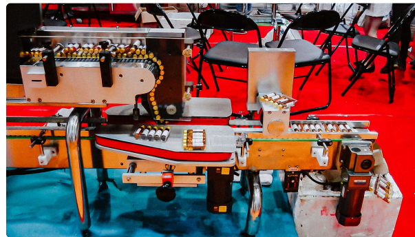
Automatic equipment for packing penicillin vials into plastic blister corks
