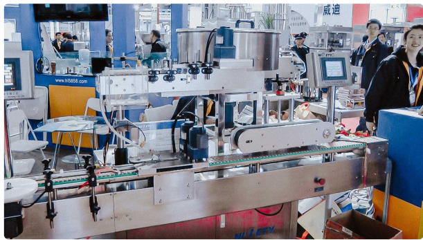
High speed automatic capping machine plastic cap for plastic bottle
