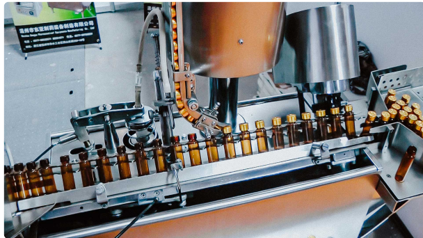
Compact model of pharmaceutical bottling and capping equipment glass vial
