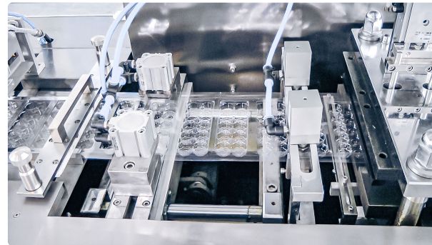
Automatic equipment for packing penicillin vials into plastic blisters in pharmaceutical...
