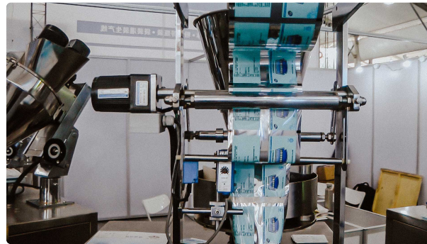
Equipment for packing bulk materials of powders granules into plastic bags Pharmaceutical Tablet Press • 03.09.2020 • 1.507K views
