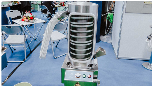
Automatic tablet dedusting machine with pharmaceutical vacuum cleaner
