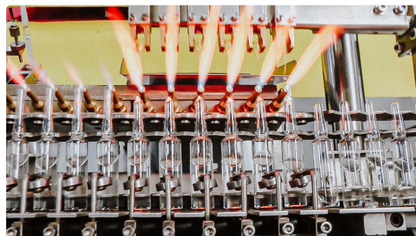
Automatic glass ampoule filling and capping line with medicine
