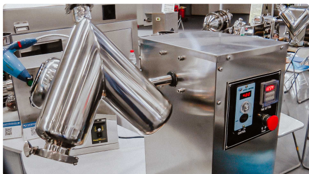
V-mixer for mixing powders in the pharmaceutical laboratory and blending...
