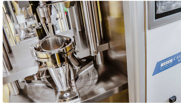
Three color layer tablet powder pressing equipment Europe Pharmaceutical Tablet Press • 07.09.2020 • 980 views
