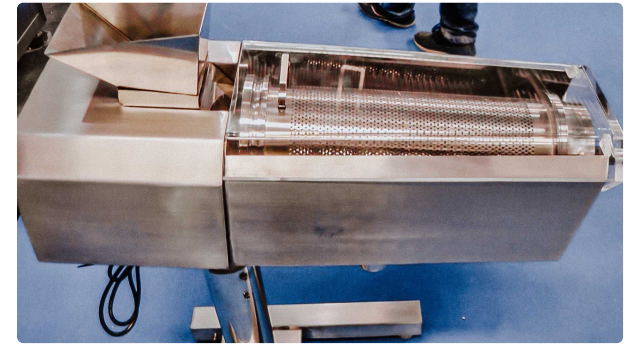
Automatic surface dust removal machine hard gelatin capsules vacuum cleaner Pharmaceutical Tablet Press • 07.09.2020 • 700 views
