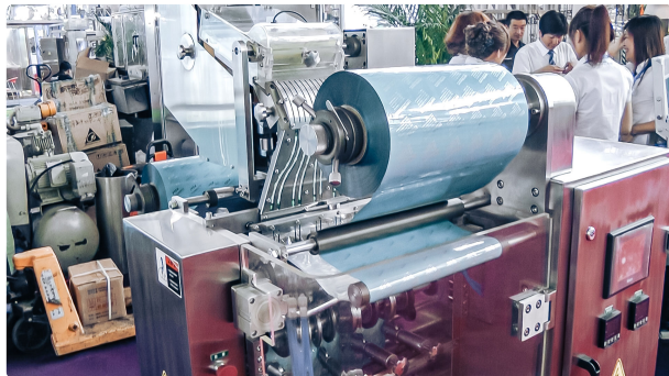
Automatic equipment for tablet packing in soft aluminum packaging in pharmaceutical...
