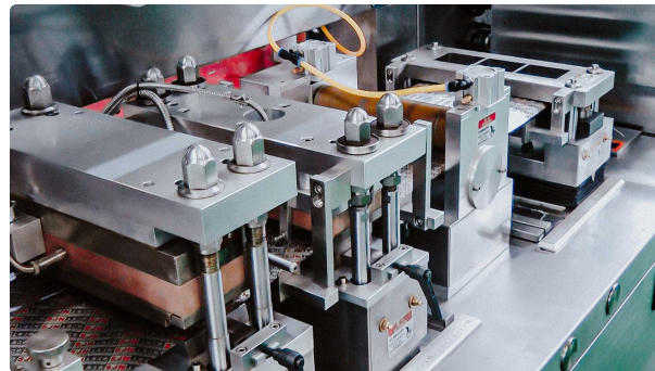
Automatic packaging machine for solid gelatin capsules and tablets in PVC Alu blisters
