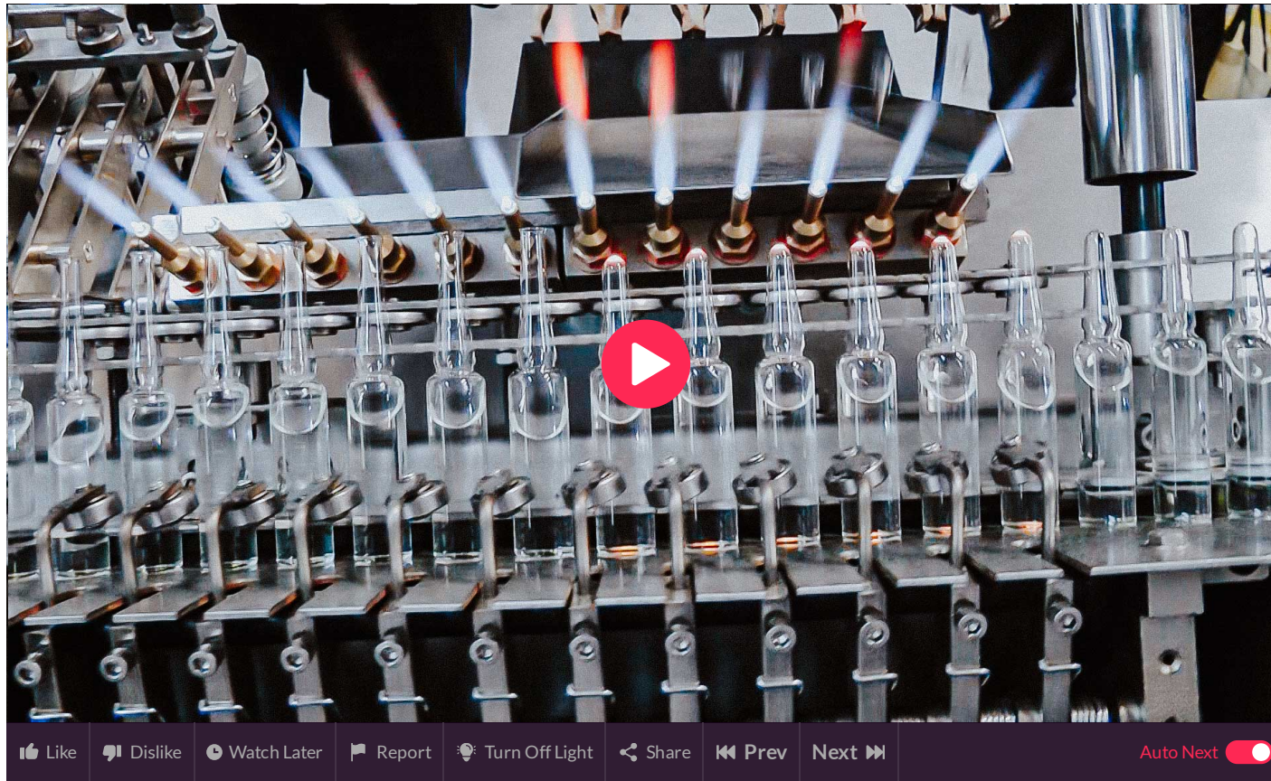
Automatic filling and sealing machine for glass ampoules with pharmaceutical drugs
