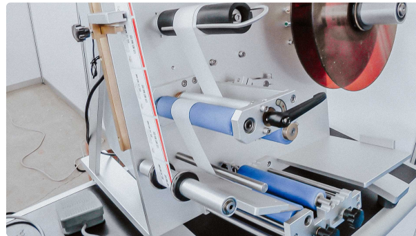
Desktop labeling machine for self-adhesive labels on plastic bottles with pharmacy products
