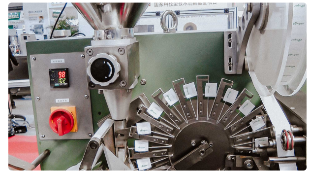
Packing machine for packing tea in filter paper bags with thread and label
