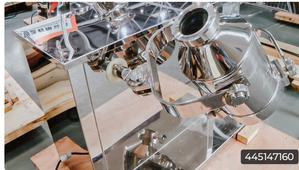
Drunk barrel mixer for powders pharmaceutical tablet production
