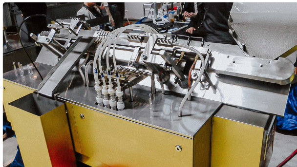
Automatic filling and closing line for penicillin bottles, rubber stoppers and aluminum caps
