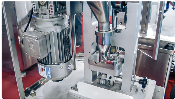
Automatic tablet production equipment with laboratory press in pharmaceutical production
