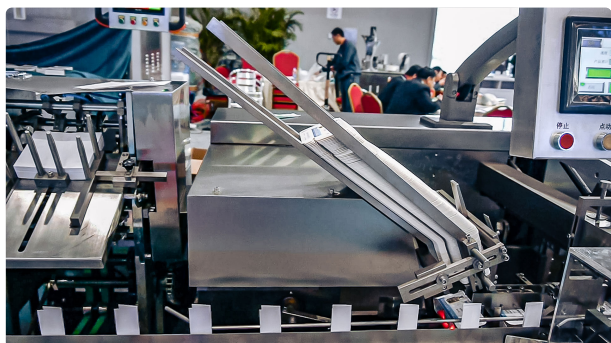
Automatic equipment for packing blisters with capsules in carton boxes
