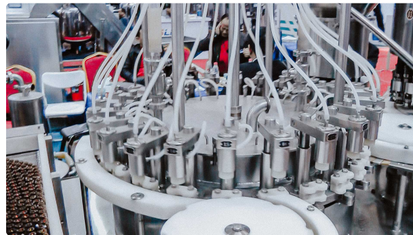
High speed automatic bottling and capping machine penicillin bottles with medicine
