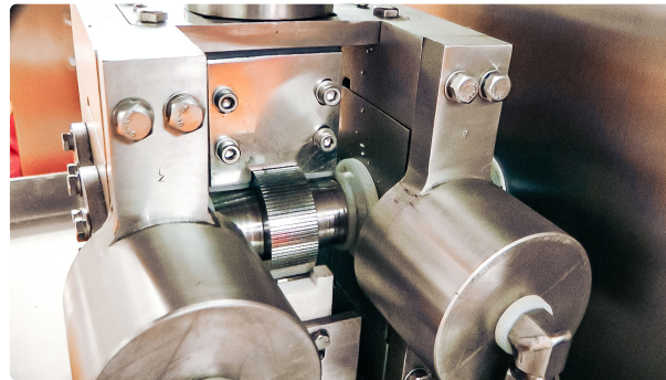
Automatic equipment for dry granulation of pellets in pharmaceutical production
