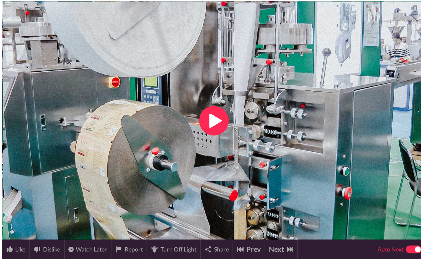
Automatic high speed packing machine for packing tea in filter bag and plastic envelope
