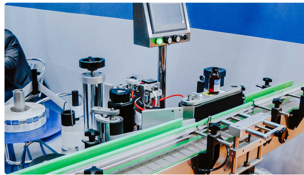
Automatic labeling machine for sticking self-adhesive labels on glass bottles with syrup
