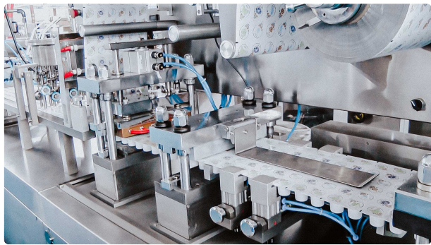
Automatic blister equipment for dispensing and packing disposable cream into blisters Europe
