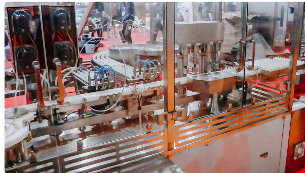
Automatic line for bottling and capping in plastic bottles with plastic cap
