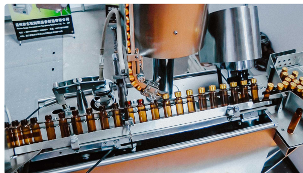
Compact model of pharmaceutical bottling and capping equipment glass vial
