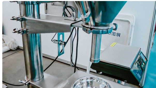
Automatic equipment for dosing powder by weight in plastic bottles
