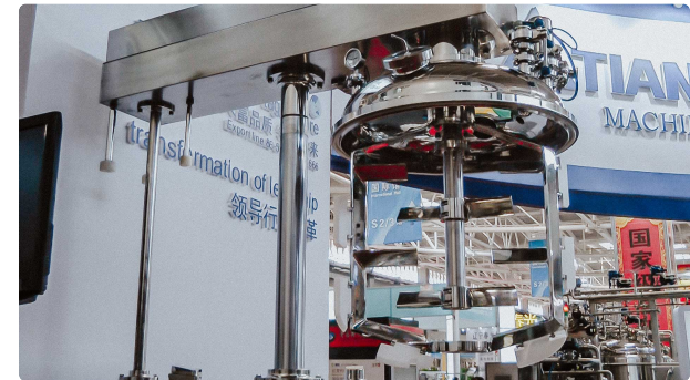
Homogenizer preparation of gel, creams and ointments for cosmetics and pharmaceuticals
