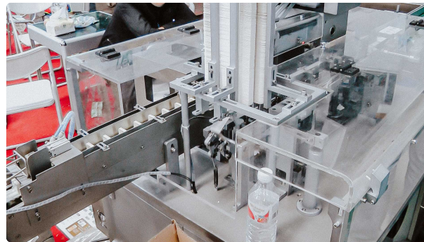
Automatic cardboard packaging machine for blisters with tablets in boxes
