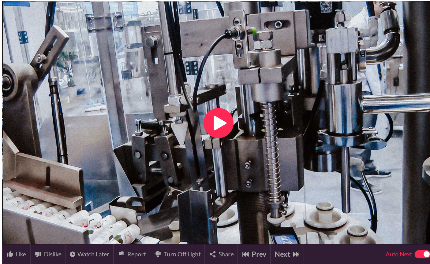
Automatic equipment for dosage and filling in plastic tubes cosmetics and pharmaceuticals cream
