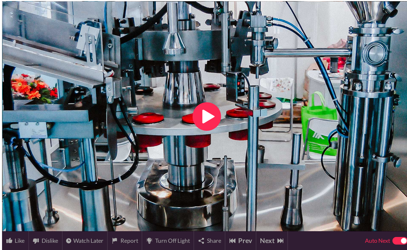
Automatic equipment for dosing and filling of plastic tubes with cream
