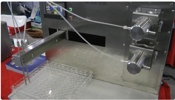
Robot for filling penicillin bottles with liquid in a cassette
