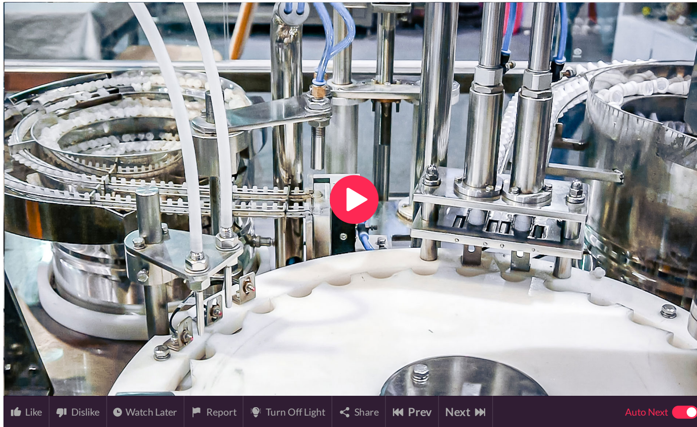
Automatic equipment for filling and closing of penicillin bottles aluminum caps
