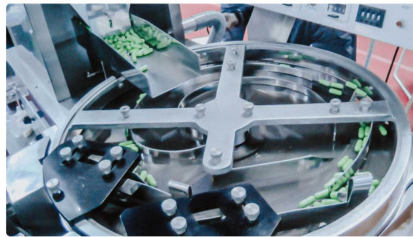
Counting and packaging of gelatine capsules in plastic bottles desktop equipment
