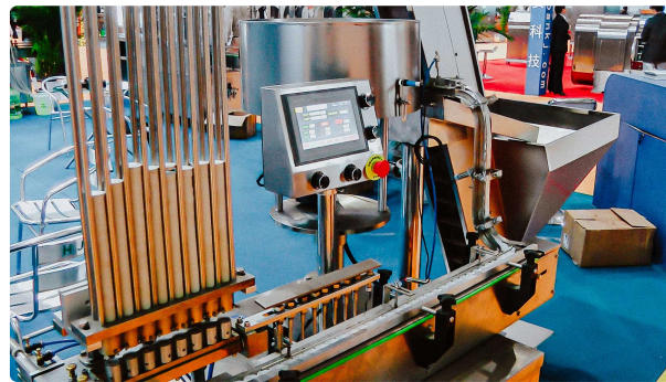
Automatic machine for packing in plastic caps aluminum membrane for welding to the bottle...
