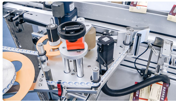
Automatic equipment for sticking self-adhesive labels on cardboard boxes of pharmaceutical...
