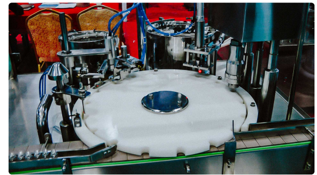
Automatic equipment for bottling and capping of 20 ml glass bottles and capping with screw...
