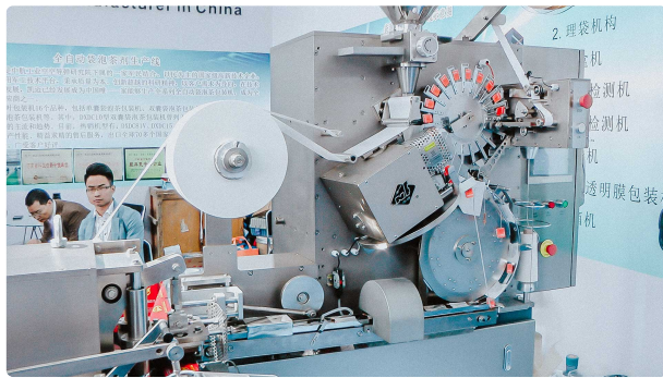
Tea packaging machine in filter paper with thread and paper label
