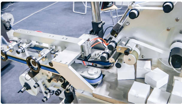
Automatic labeling equipment for labelling in pharmaceutical production
