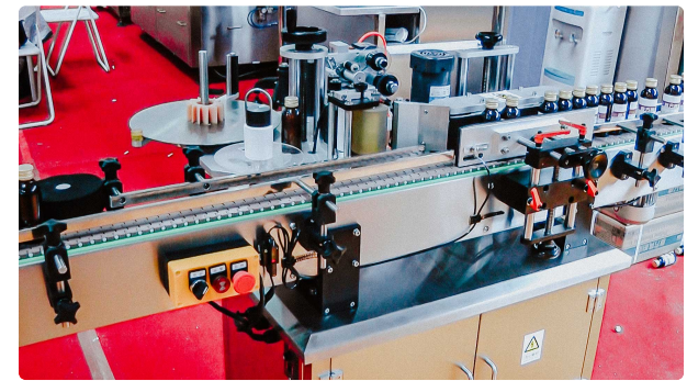
Automatic labeling machine for labeling glass medicine bottles
