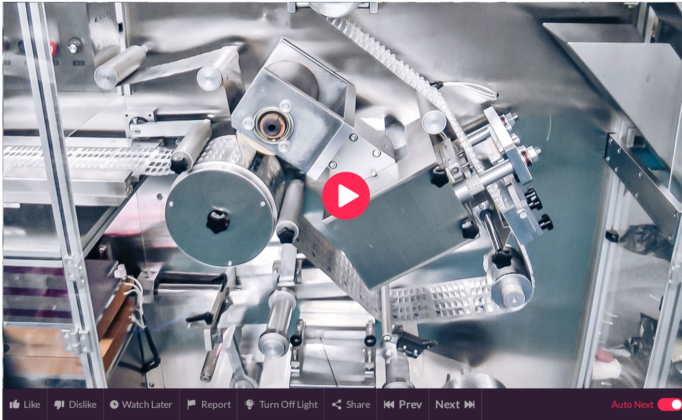
Automatic equipment for PVC/ALU blister capsules packaging in pharmaceutical production
