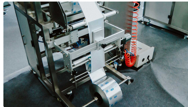
Automatic powder dispensing machine for packing plastic pillow bags Pharmaceutical Tablet Press • 11.09.2020 • 1.220K views
