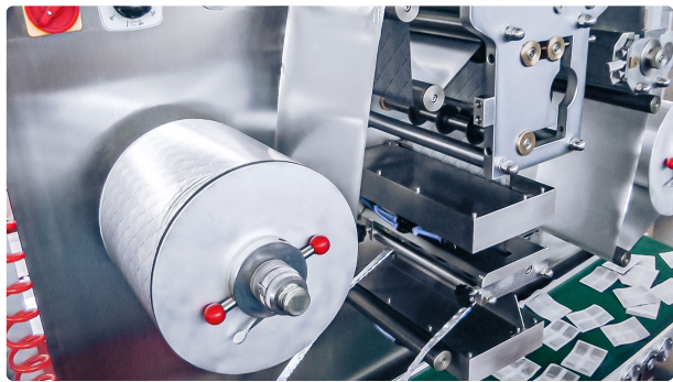
Automatic equipment for group packaging of tablets in aluminum tape pharmaceutical...
