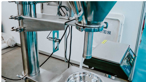
Automatic equipment for dosing powder by weight in plastic bottles
