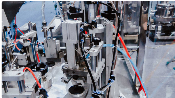
Tube-filling machine for automatic cream filling of plastic tubes
