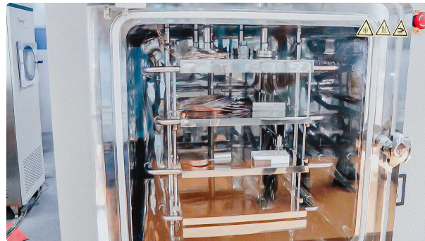
Sublimation lyophilic dryer for powder production from food and pharmaceutical...
