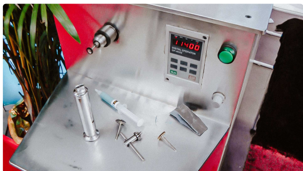
Polishing metal surface of the punch and matrix for pressing tablets
