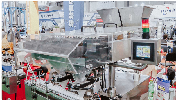
Counting and packing machine for packaging tablets and gelatin capsules in plastic bottles...
