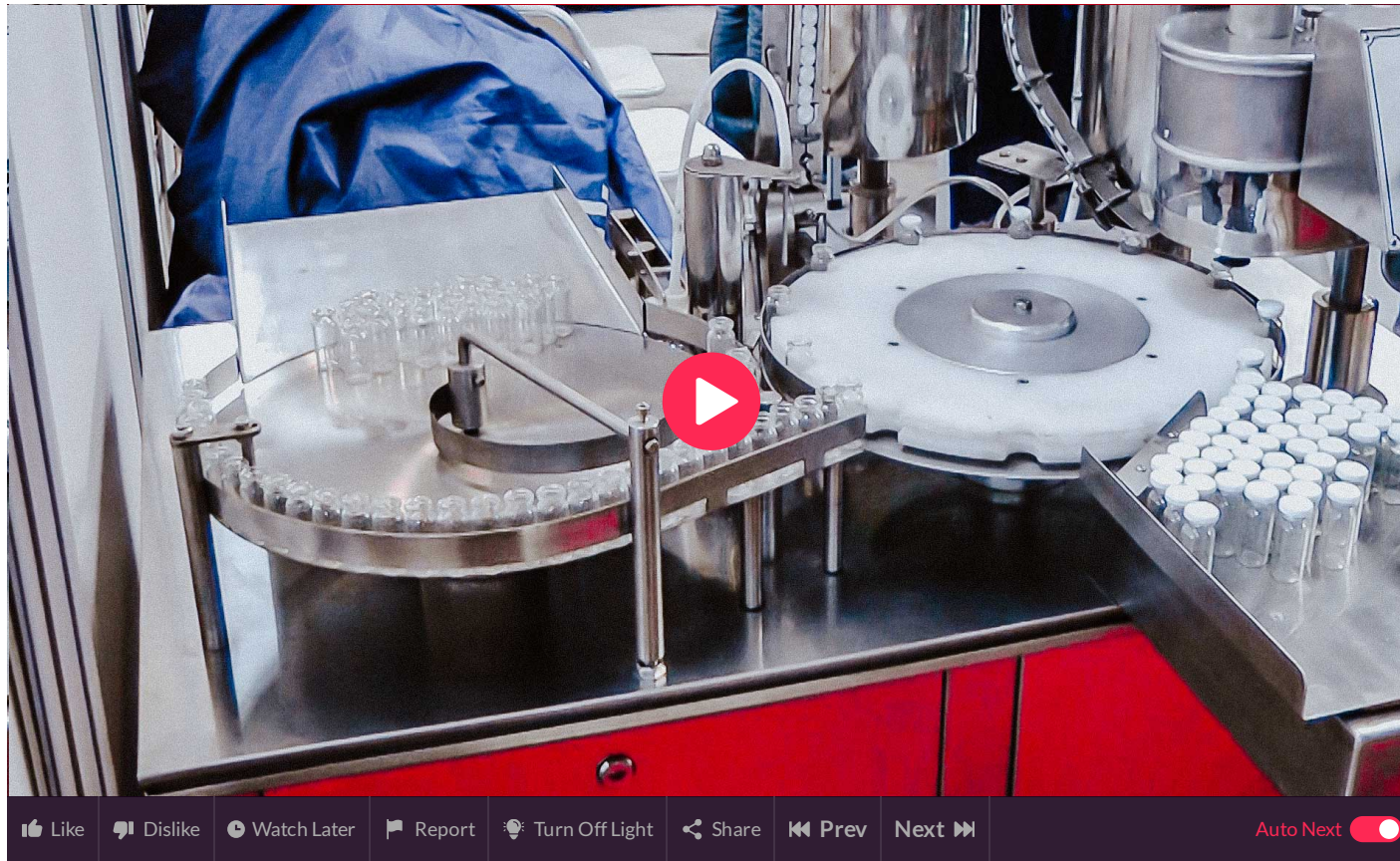
Automatic penicillin bottle filling and capping machine and aluminum caps
