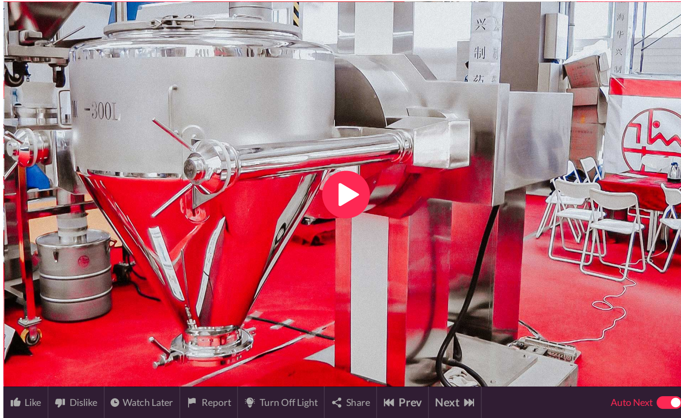
Pharmaceutical cone mixer of powders and granules in the production of medicines
