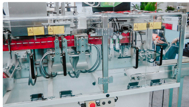
Automatic line for the production of wet wipes with alcohol individual package USA
